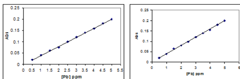
Calibration curve for lead (atomic absorption method) Calibration curve for lead (spectroscopic method)
