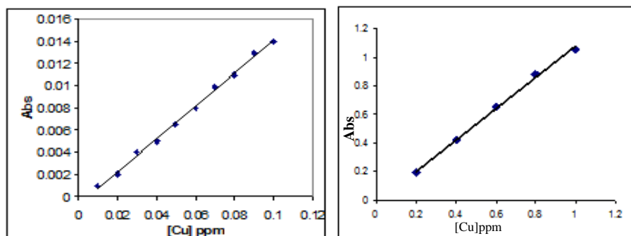
Calibration curve for copper (Atomic absorption method) Calibration curve for copper (spectroscopic method)
