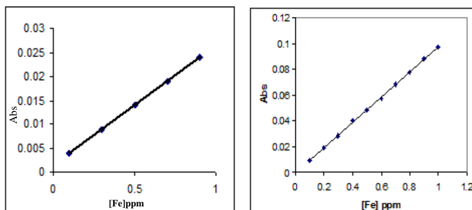
Calibration curve for Iron (Atomic absorption method) Calibration curve for Iron (spectroscopic method)
