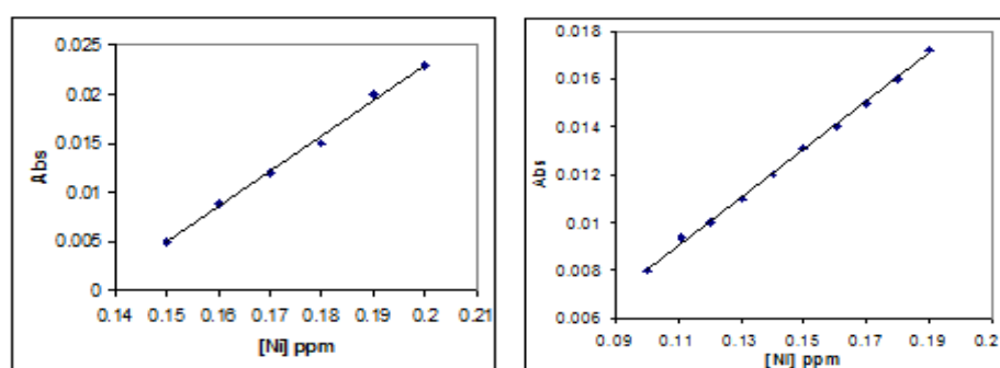
Calibration curve for nickel (Atomic absorption method) Calibration curve for nickel (spectroscopic method)
