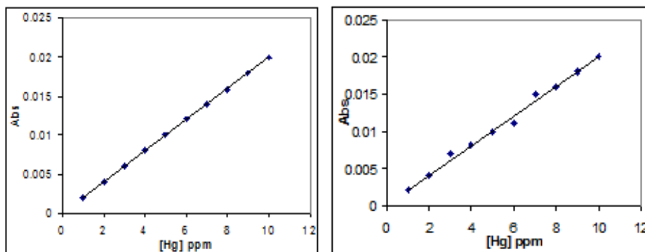
Calibration curve for mercury (atomic absorption method) Calibration curve for mercury (spectroscopic method)
