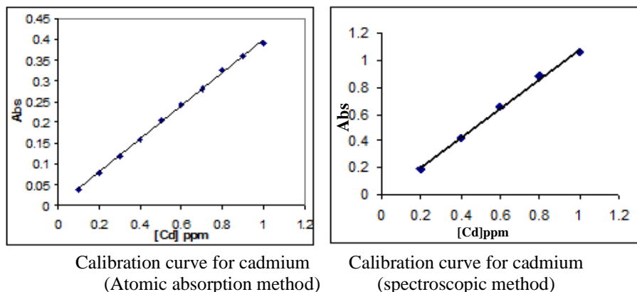
Fig. 3. Calibration curves for the ion cadmium
