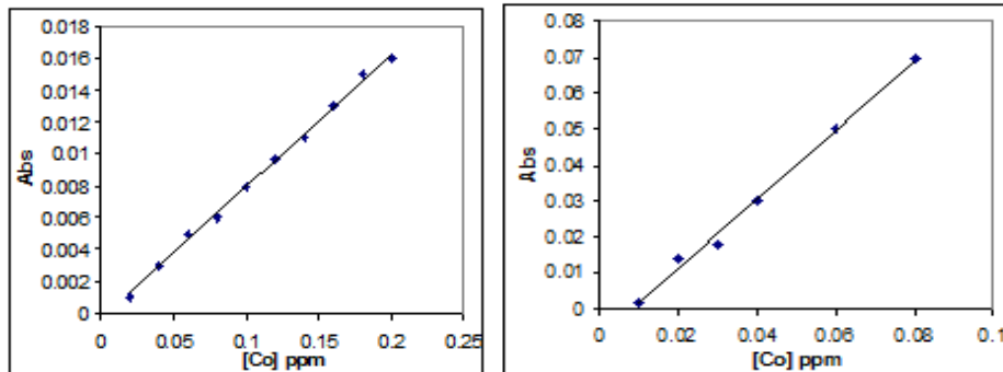
Calibration curve for cobalt (Atomic absorption method) Calibration curve for cobalt (spectroscopic method)
